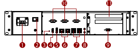
Rear side I/O
